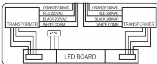
208/220/240 VOLT (DUAL CIRCUIT):
