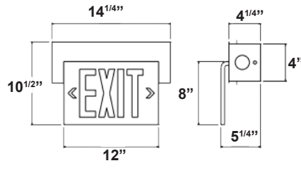
Recessed Wall
