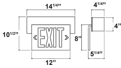
Surface Wall
