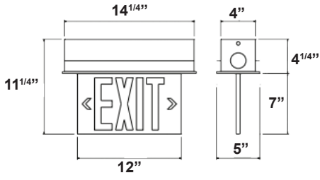
Recessed Ceiling
