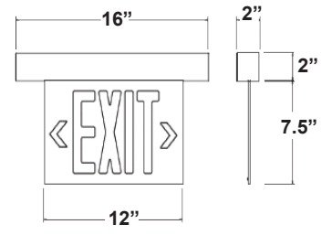
Mullion Mount
