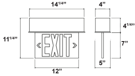
Surface End
